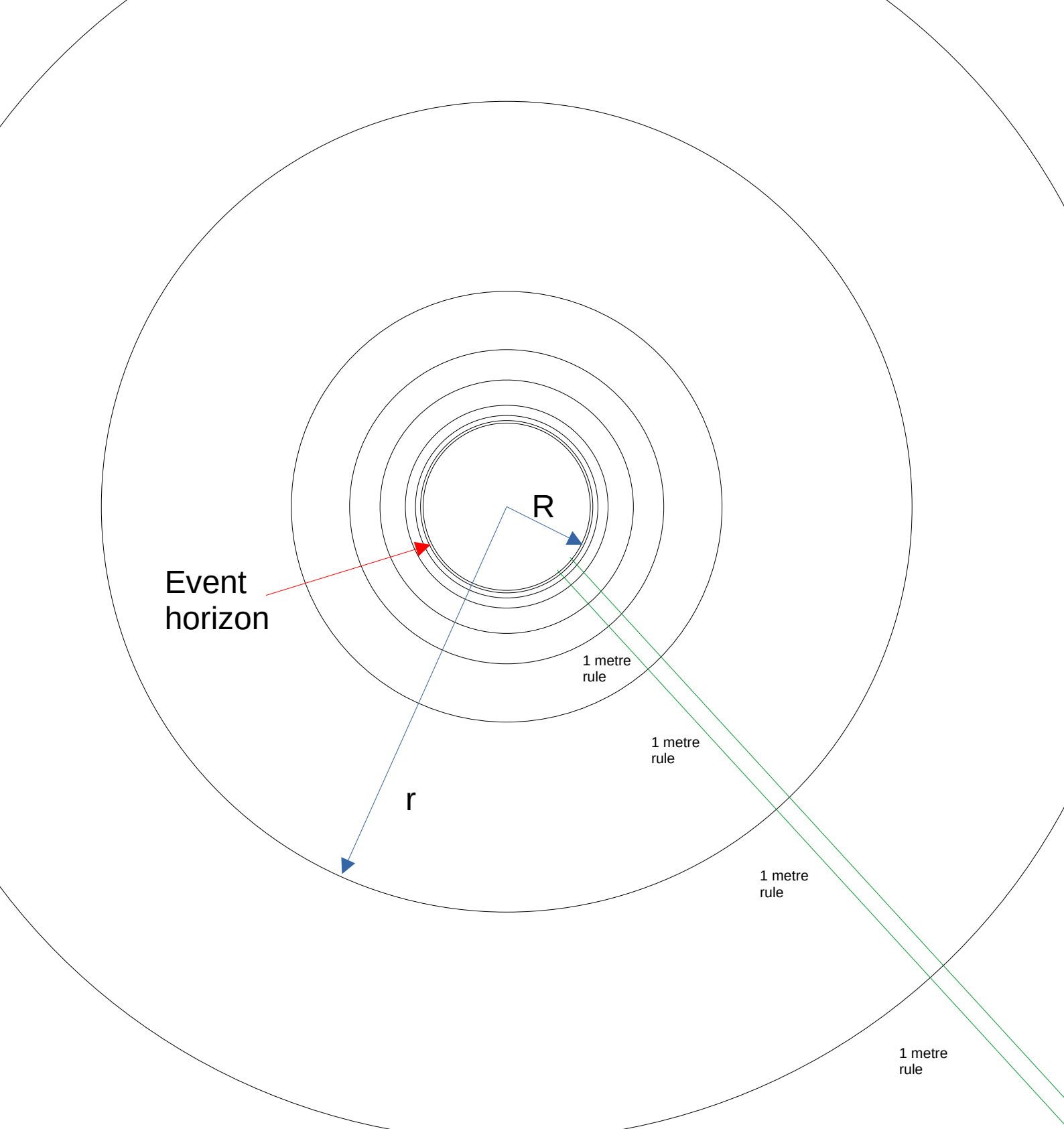
The Schwarzschild metric round a mass in an otherwise empty Universe
