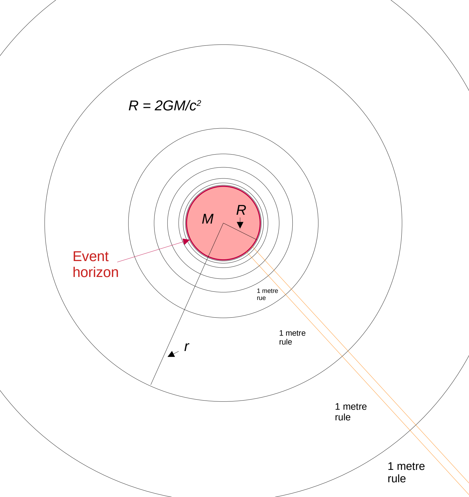
The Schwarzschild metric round a mass, M , and with an event horizon at a radius, R
