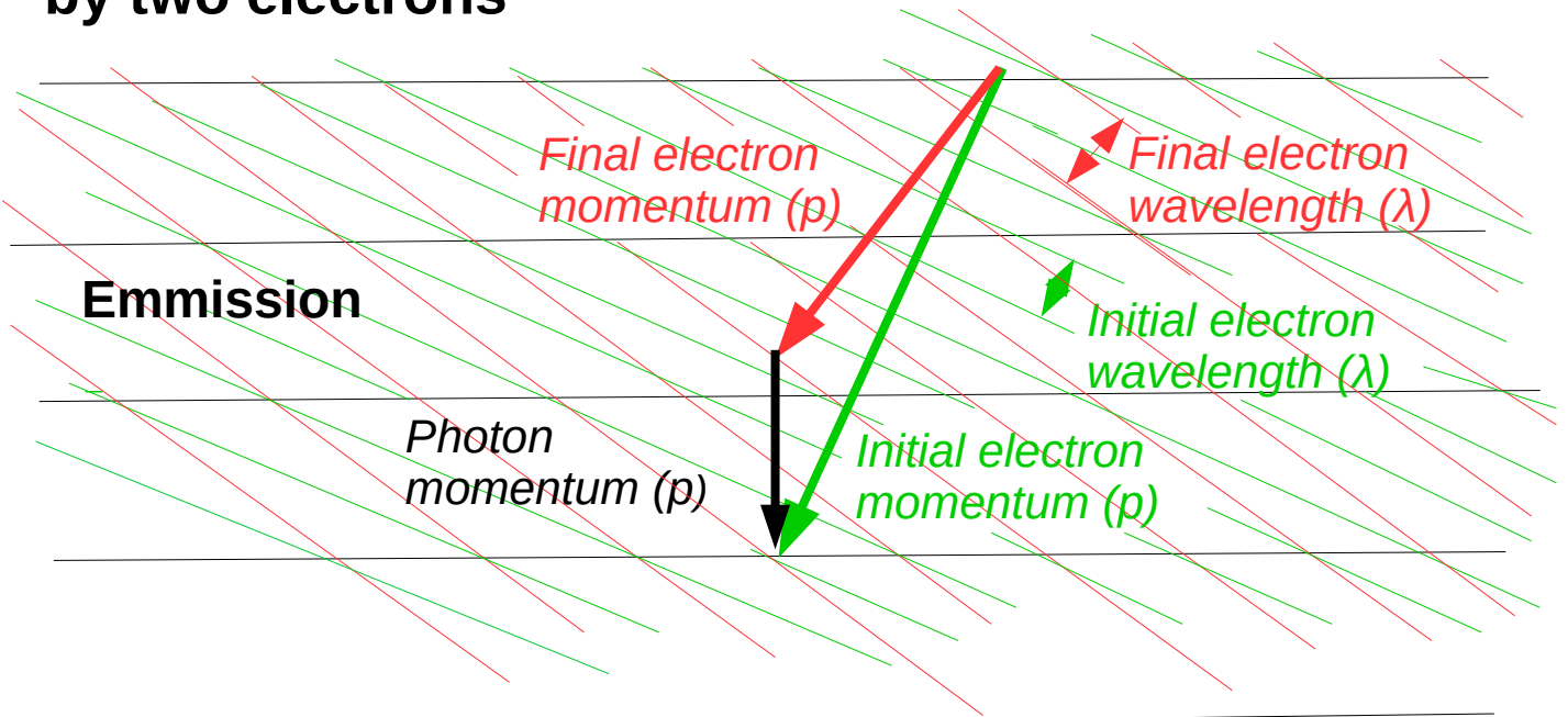
Figure 7. The emission and absorption of a photon by two electrons
